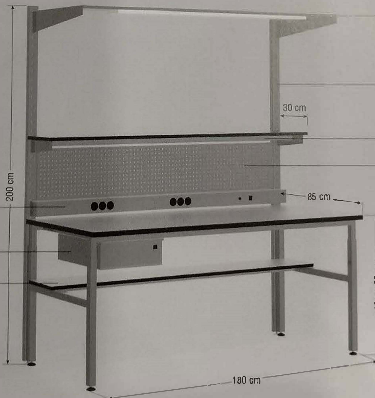
WORKBENCH - STANDARD AND ESD VERSION WITH ACCESSORIES
